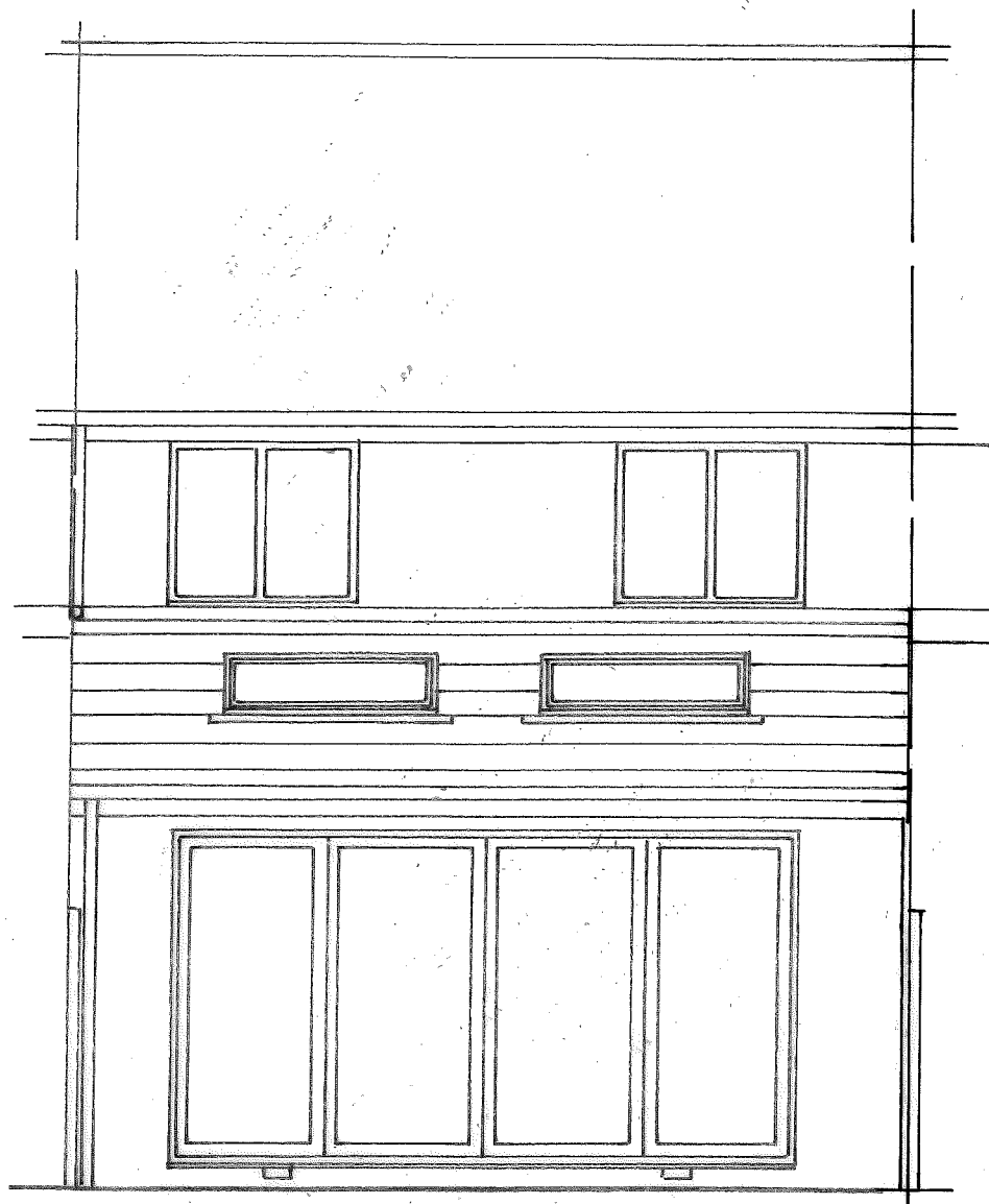
PROPOSED REAR 1:50
